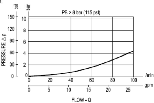
By-pass line pressure drop
