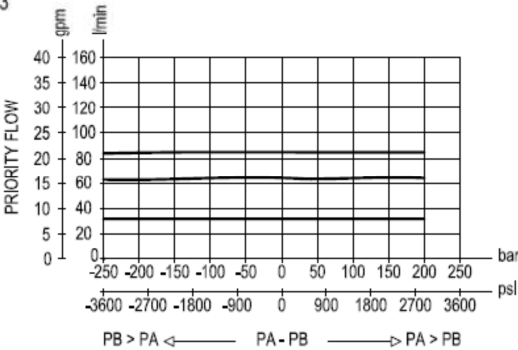
Priority Flow vs Pressure
