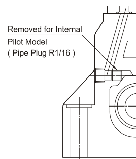
Section Y-Y
