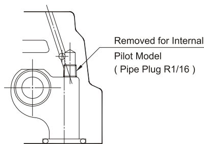
Section X-X
