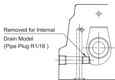
Section Y-Y
