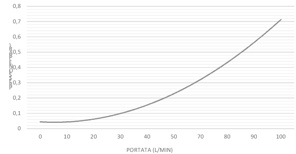
FILTER HOUSING PRESSURE DROP (IN/OUT 3/4")
