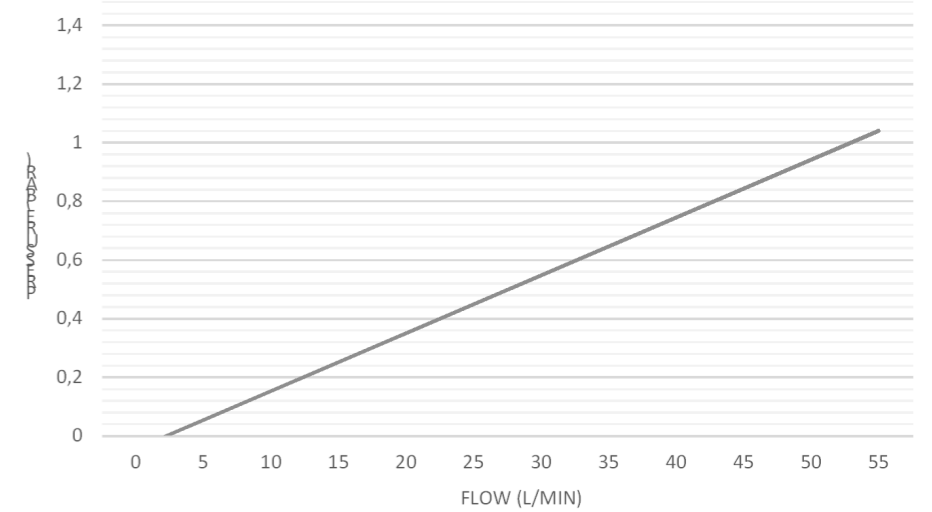
FILTER HOUSING PRESSURE DROP (IN/OUT 3/4")
