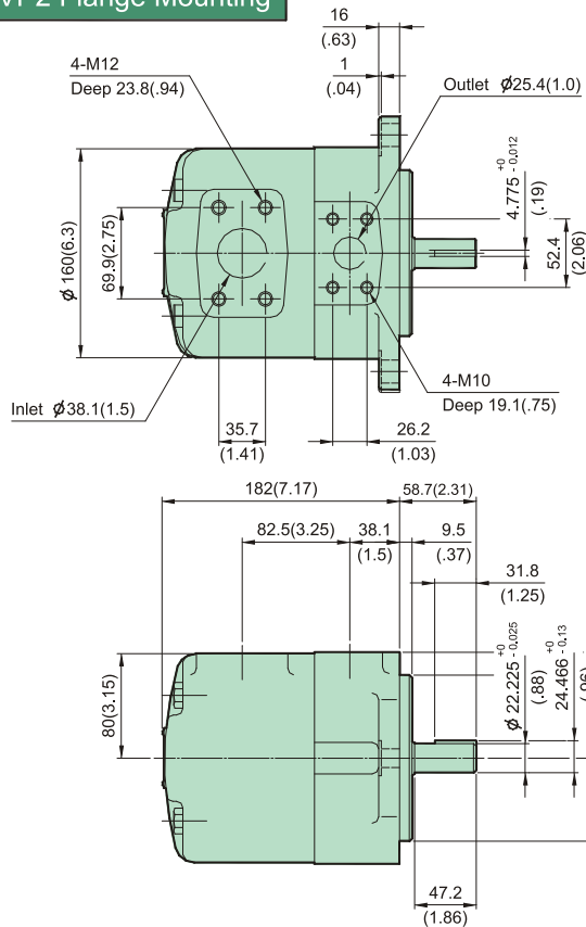
IVP2 Flange Mounting
