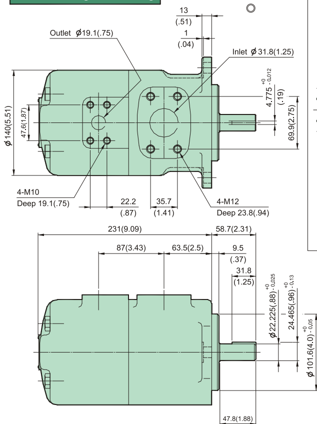
IVPQ1 Flange Mounting
