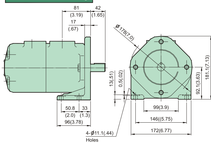
IVPQ1 Foot Mounting
