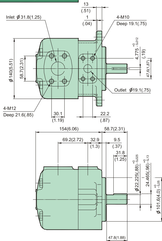
IVP1 Flange Mounting
