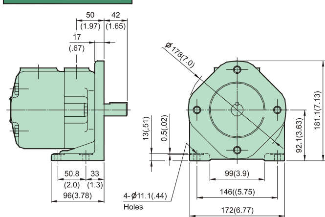
IVP1 Foot Mounting
