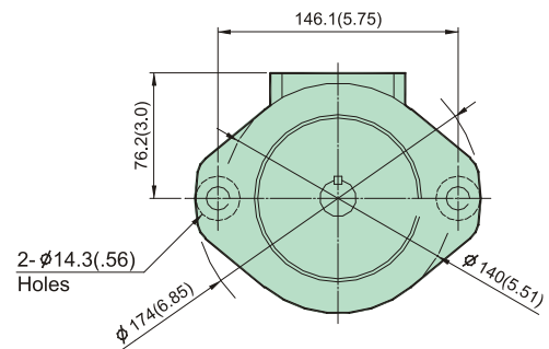
IVPQ1 Foot Mounting
